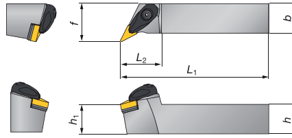
Enlarged view of 2020 type Right hand (R) shown.
